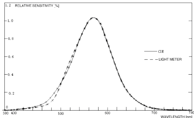
Spectral sensitivity characteristic curve.
