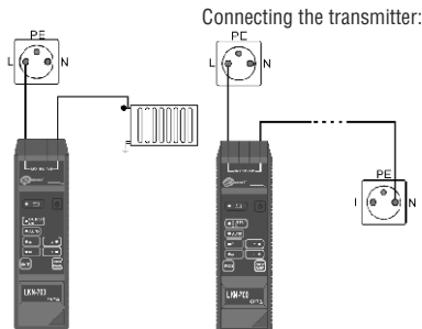
Connecting the transmitter:
