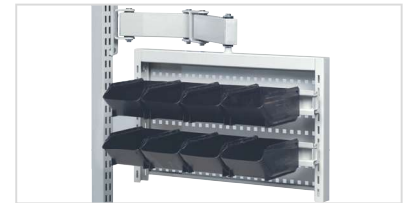
Rotating tool panel frame with M500 perforated panel, M500 bin rails and 8 plastic ESD bins
